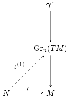
FIGURE 10. Dual tautological bundle pulls back to an immersed submanifold.
