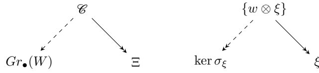
FIGURE 12. The rank-one variety \mathcal{E} is the incidence correspondence for the characteristic scheme \Xi .
